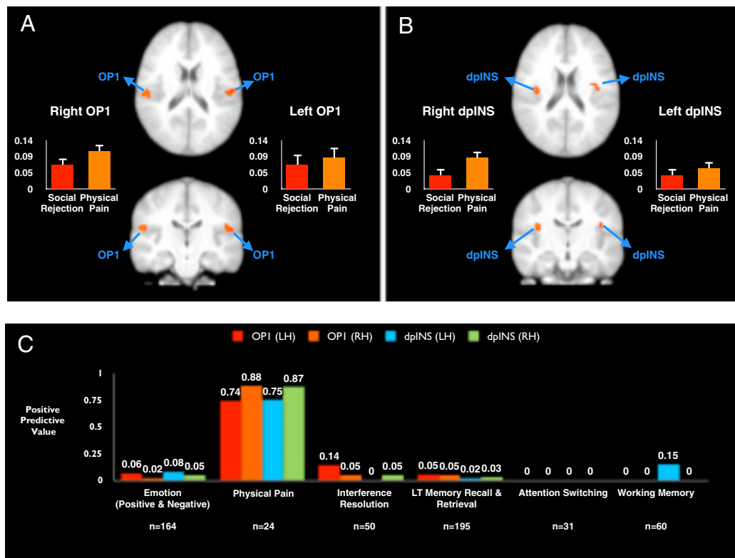
Fig. 3. Operculo-insular ROI analyses. The neural overlap between social rejection and physical pain in (A) OP1 [right hemisphere (RH): 46 voxels; x = 56, y = -23, z = 21, t_{\text{peak}} = 3.52 ; left hemisphere (LH): 43 voxels; x = -48, y = -17, z = 21, t_{\text{peak}} = 2.97 ] and (B) dpINS (RH: 24 voxels; x = 39, y = -15, z = 18, t_{\text{peak}} = 2.85 ; LH: 23 voxels; x = -39, y = -9, z = 23, t_{\text{peak}} = 2.75 ). Coordinates are in Talairach space. Bar graphs demonstrate the \beta -values for social rejection and physical pain in each ROI. Error bars represent one SE. We performed two separate repeated-measure ANOVAs using the \beta -values extracted from OP1 (Analysis #1) and dpINS (Analysis #2) ROIs. Each analysis included pain type (social vs. physical) and hemisphere (right vs. left) as within participant factors. These analyses revealed no significant main effects (OP1: all F < 0.84 , all P > 0.36 ; dpINS: all F < 2.64, P > 0.11 ) or interactions (OP1: F = 0.31, P = 0.58 ; dpINS: F = 2.25 , all P > 0.14 ). These findings indicate that it was not the case that one type of pain led to significantly greater activation compared with the other, or that the activations were lateralized to one side of the brain in these ROIs. (C) Bar graphs illustrating the results of a Bayesian analysis, which examined the specificity of the activation observed in OP1 (RH: x = 56, y = -23, z = 21 ; LH: x = -48, y = -17, z = 21 ) and dpINS (RH: x = 39, y = -15, z = 18 ; LH: x = -39, y = -9, z = 23 ) for physical pain. Bars represent the probability that a study activating a region within 10 mm of the peak coordinate in OP1 (red and orange bars) and dpINS (blue and green bars) belonged to that task category (i.e., the positive predictive value for each task type). Error bars represent one SE. “ n ” refers to the number of each type of study included in the meta-analysis.
